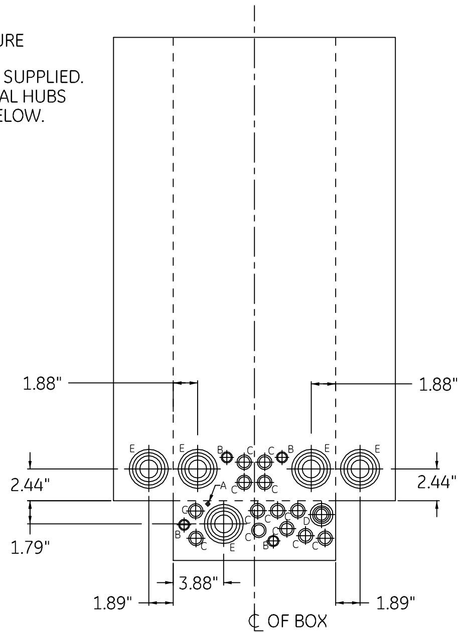
KNOCKOUT DIAGRAM
