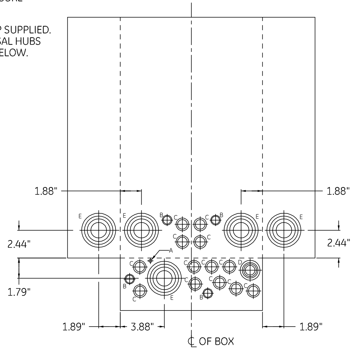
KNOCKOUT DIAGRAM
