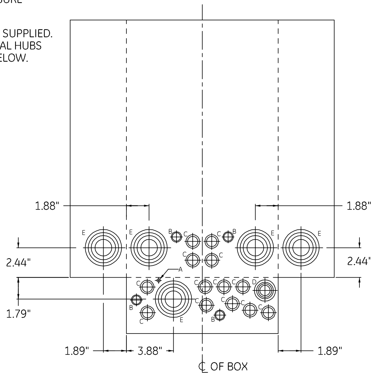
KNOCKOUT DIAGRAM
