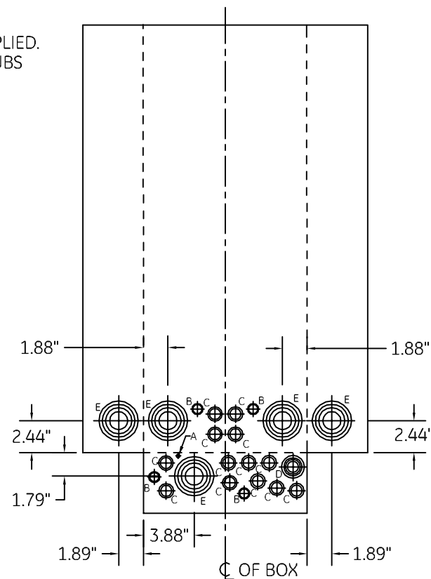
KNOCKOUT DIAGRAM
