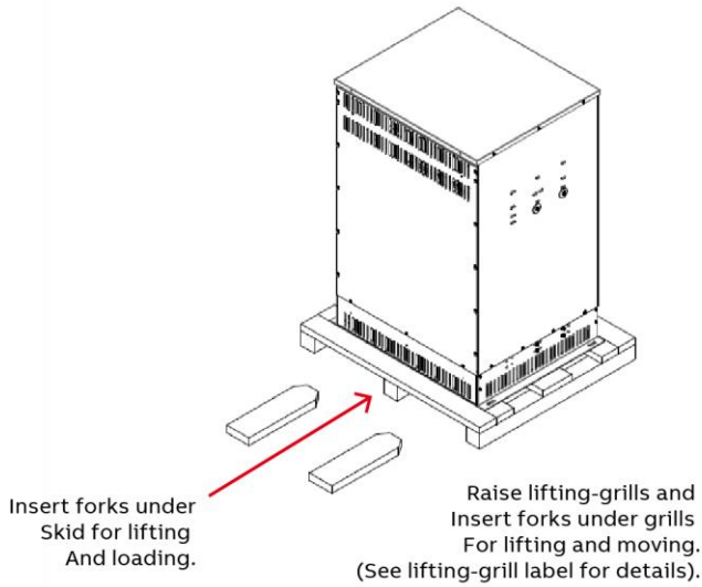
Fig.1 (With Shipping Skid)
