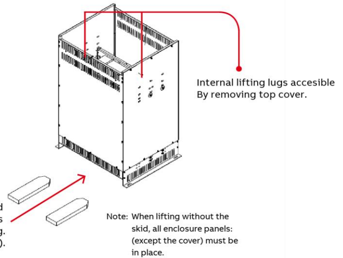
Fig.2 (Without Shipping Skid)
