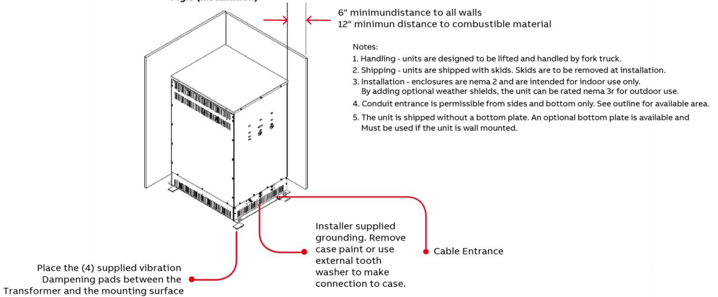
Fig.3 (Installation)
