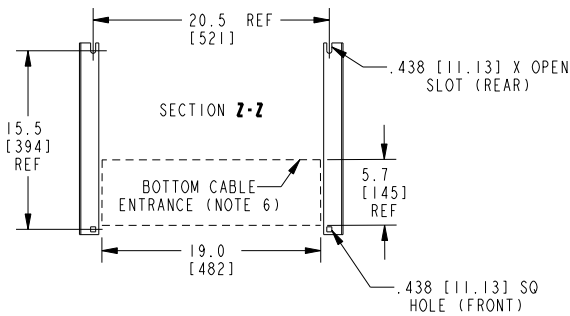
BOTTOM VIEW OF MOUNTING AND CABLE ENTRANCE
