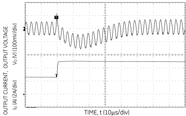
Figure 12. Transient Response to Dynamic Load Change from 50% to 100% of full load (V o = 5.0 Vdc, C ext = 2x150 µF Polymer Capacitors).
