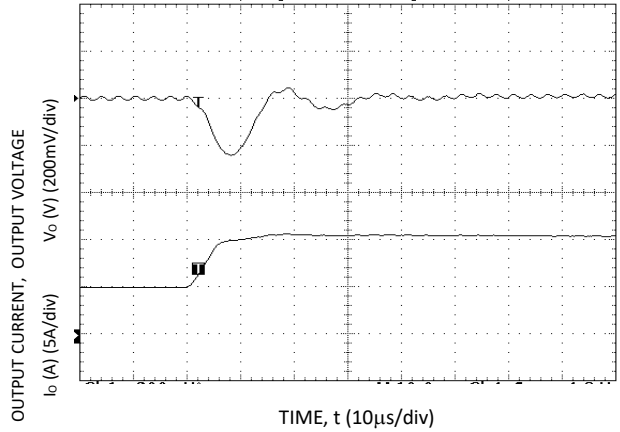
Figure 10. Transient Response to Dynamic Load Change from 50% to 100% of full load ( V_o = 3.3\text{Vdc} ).
