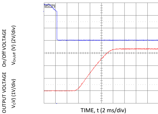
Figure 15. Typical Start-Up Using Remote On/Off with Low-ESR external capacitors ( V_{in} = 5.5\text{Vdc} , V_o = 3.3\text{Vdc} , I_o = 10.0\text{A} , C_o = 1050\ \mu\text{F} ).
