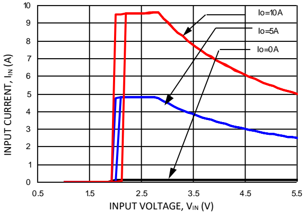
Figure 7. Input voltage vs. Input Current ( V_o = 2.5\text{Vdc} ).
