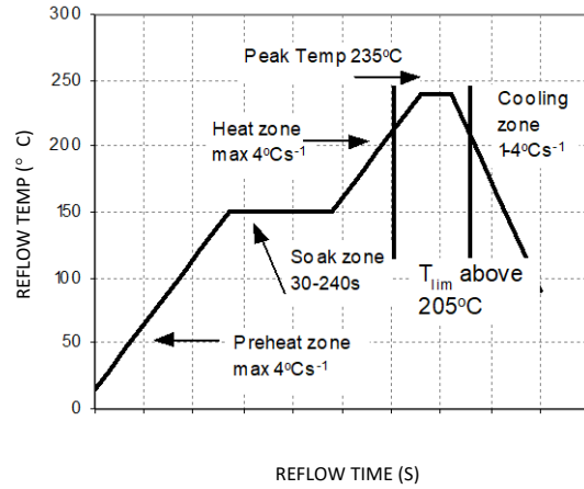
Figure 37. Reflow Profile for Tin/Lead (Sn/Pb) process.
