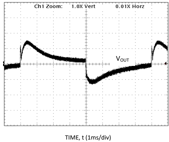
Figure 8. 12V Transient response 100 – 200A, V_{IN} = -48V_{DC} .
