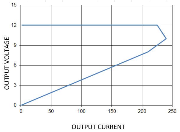
Figure 2. 12V output: Current limit profile (Vin: -48V DC )
