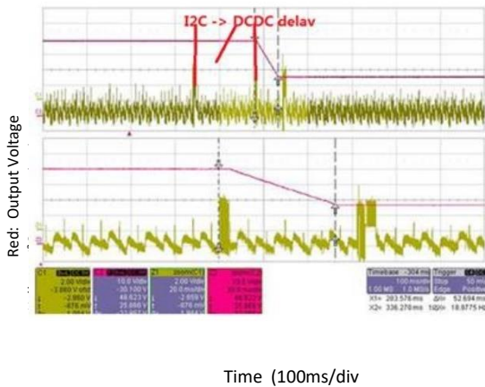
Figure 15. Turn-OFF at full load, V IN =230V AC
