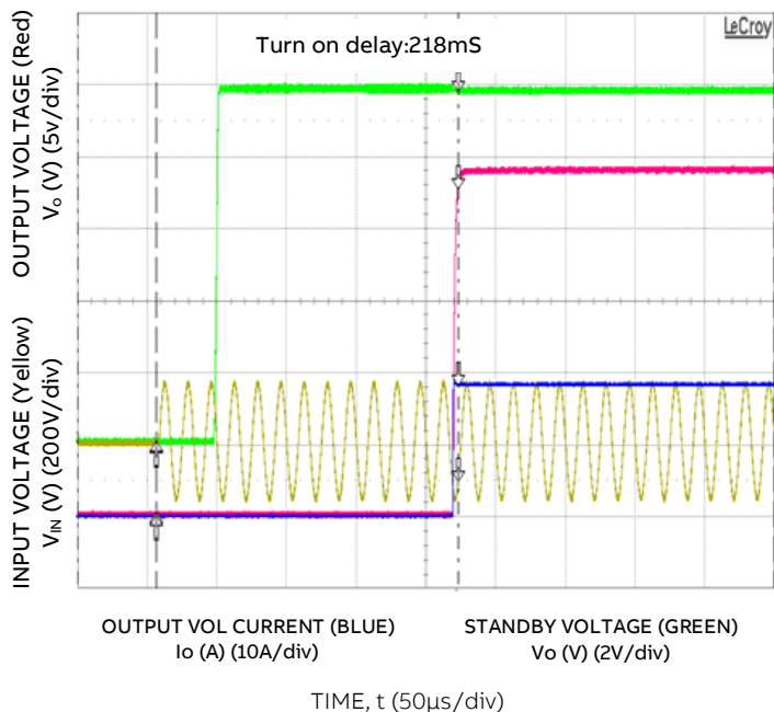
Figure 4. Typical Start-up ( V_{IN} = 115\text{Vac} , Full Load)
