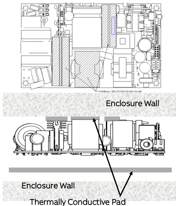
Fig 1. Example arrangement of the CLP0424/28 for sealed enclosure applications.
