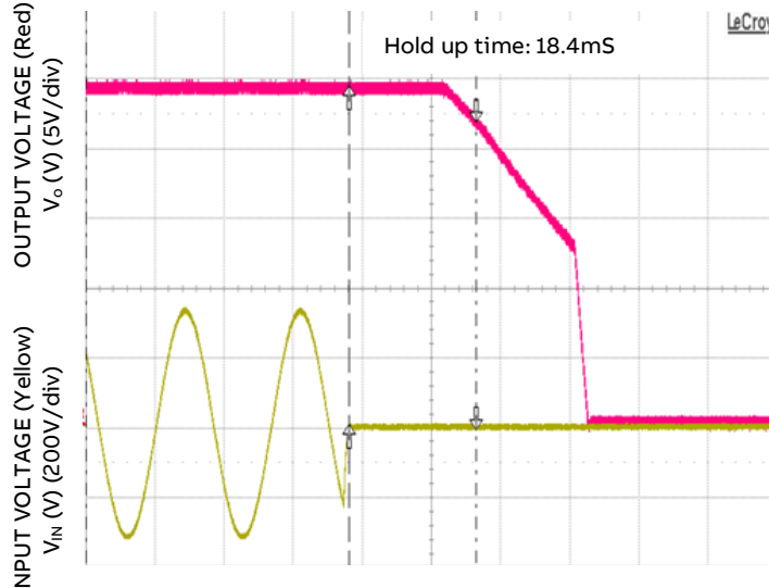
Figure 7. Typical Hold-up Waveforms ( V_{IN} = 230\text{V} , 100% Load)
