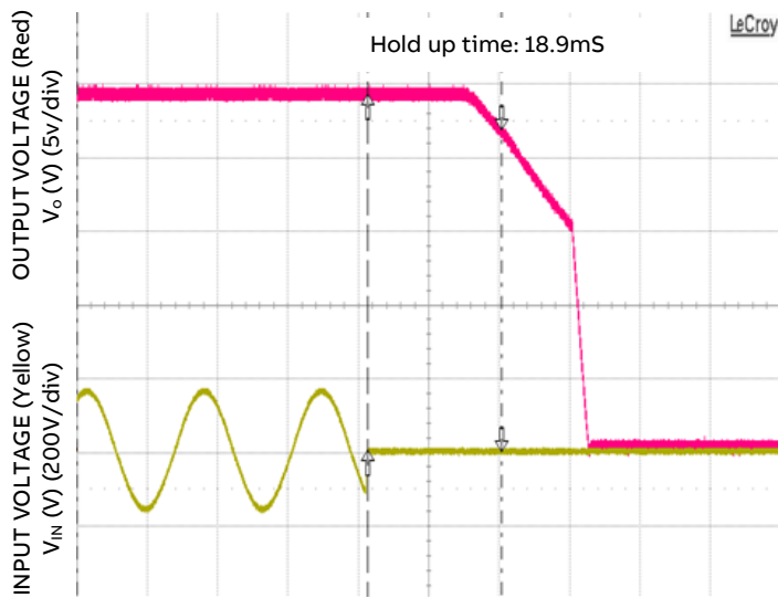
Figure 6. Typical Hold-up Waveforms ( V_{IN} = 115\text{Vac} , 100% Load)
