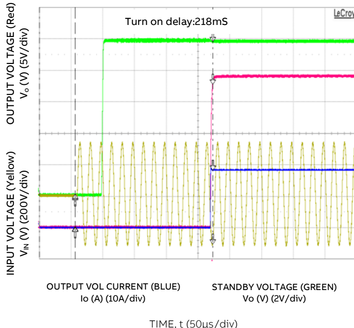
Figure 5. Typical Start-up ( V_{IN} = 230\text{V} , Full Load)
