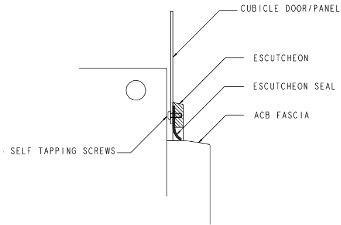
Figure 3: Door side view
