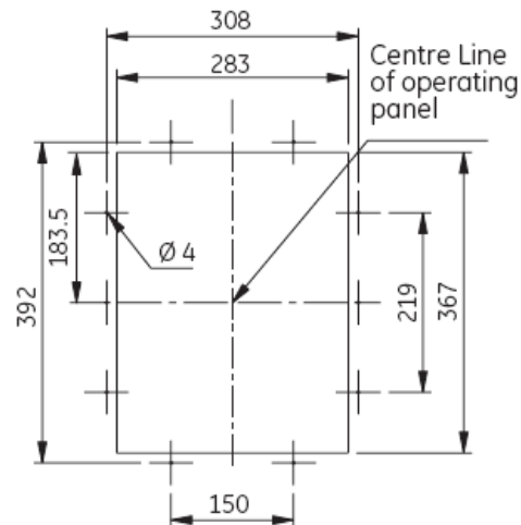
Figure 1 Cut out details for Drawout breaker
