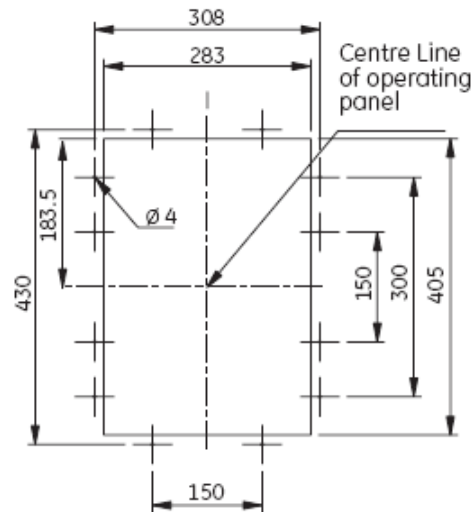
Figure 1 Cut out details for Drawout breaker
