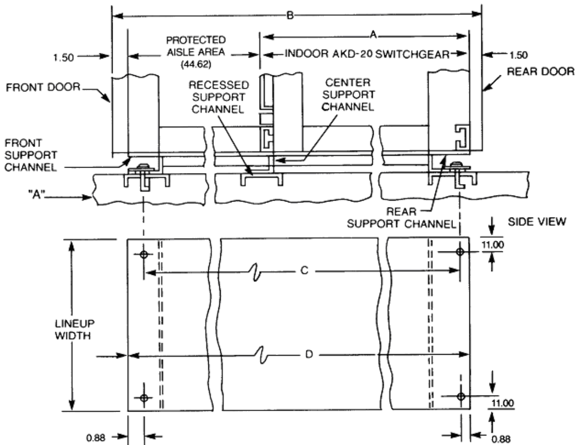
Plan view at level "A"
