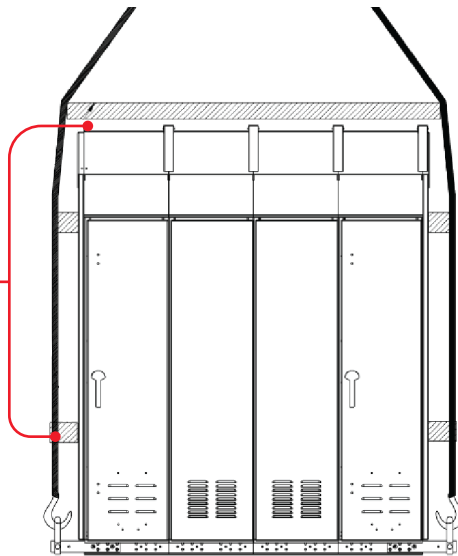
Fig. 2.5 Recommended method of lifting outdoor enclosure (using cable spreaders)
