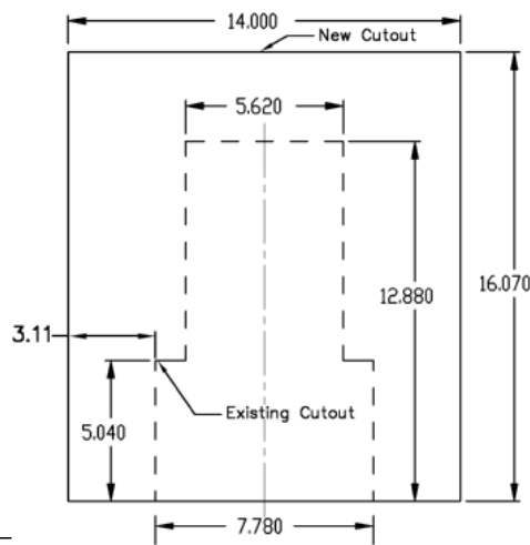
Figure 7: 2500A FC, BC, 3000A FC, and BC Panel Cutout
