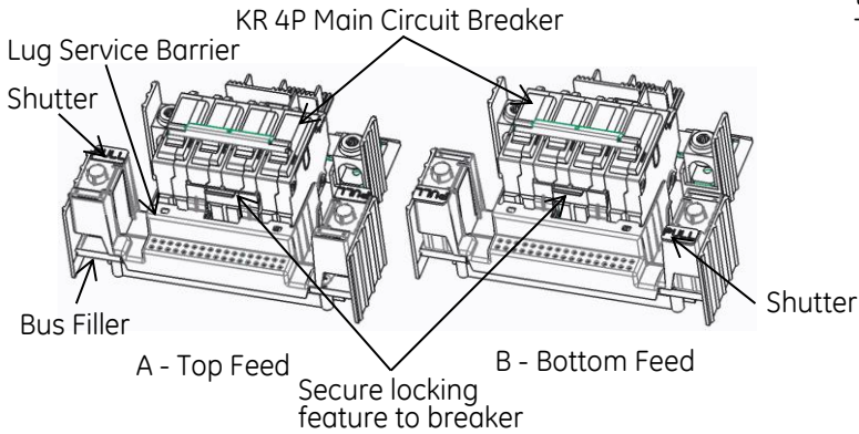
Figure 3: Fully Assembled Lug Service Barrier
