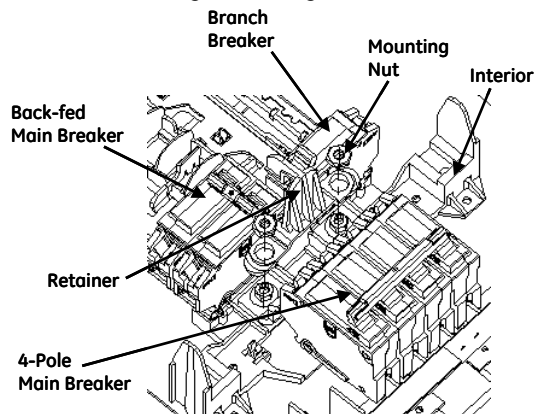
Figure 1: Main Breaker Retainer
