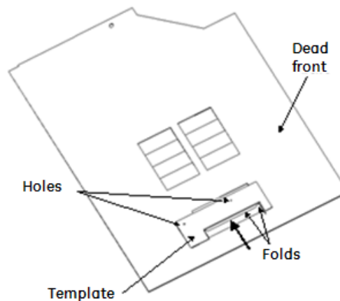
Figure 2: Mounting Hole Template
