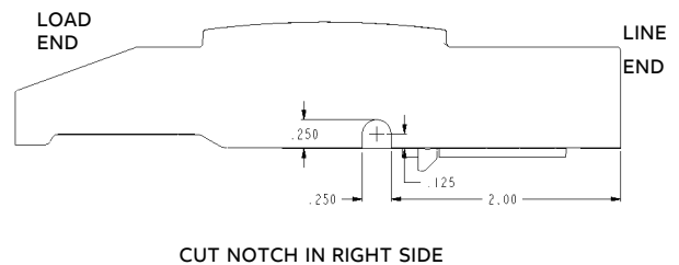
Figure 4a. Side View of Breaker Cover
