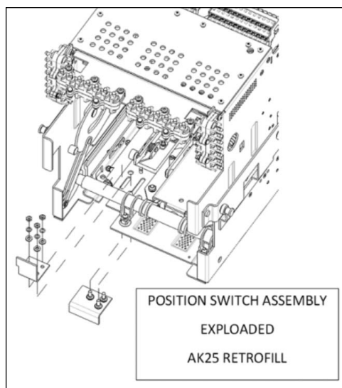
Figure 21. AKD-5, AK25 Retrofill Breaker, Actuator for Position Switch Assembly (Exploded View)
