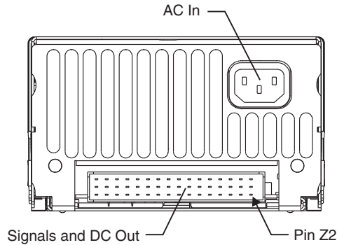
Figure 2. NP0800 Connectors
