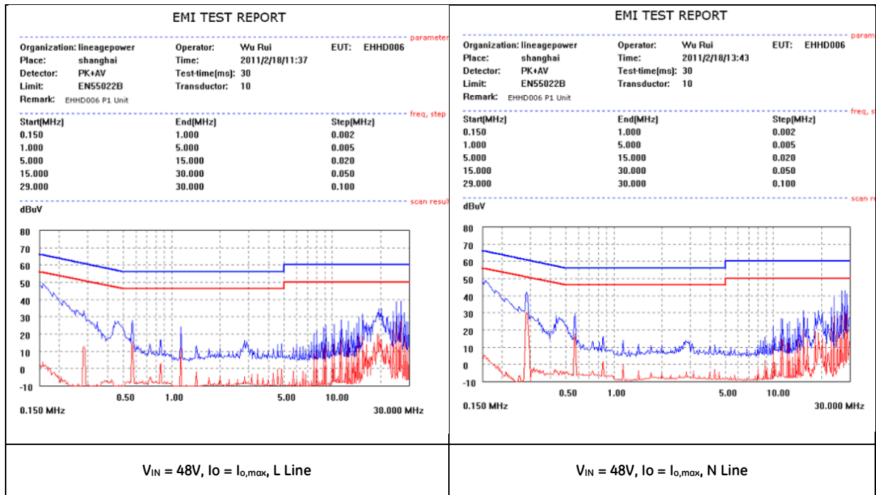
Figure 25. EMC Considerations
