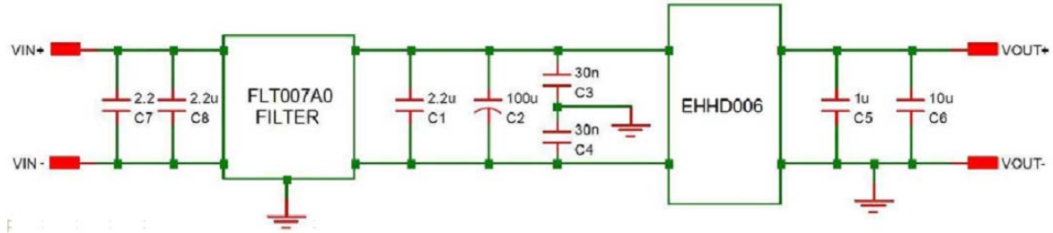
Figure 25. EMC Considerations
