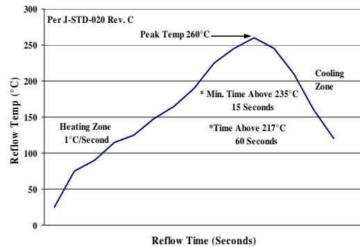
Figure 24. Recommended linear reflow profile using Sn/Ag/Cu solder.
