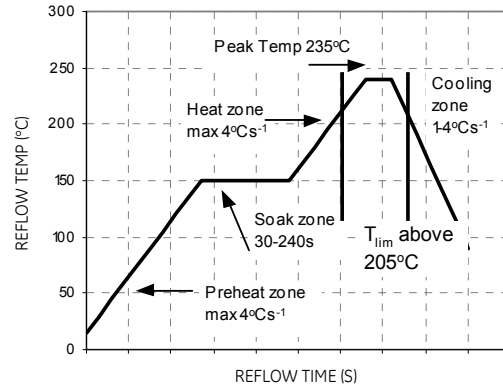
Figure 16. Reflow Profile for Tin/Lead (Sn/Pb) process.
