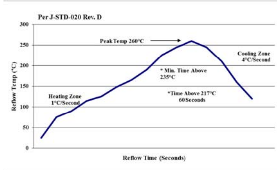
Figure 18. Recommended linear reflow profile using Sn/Ag/Cu solder.
