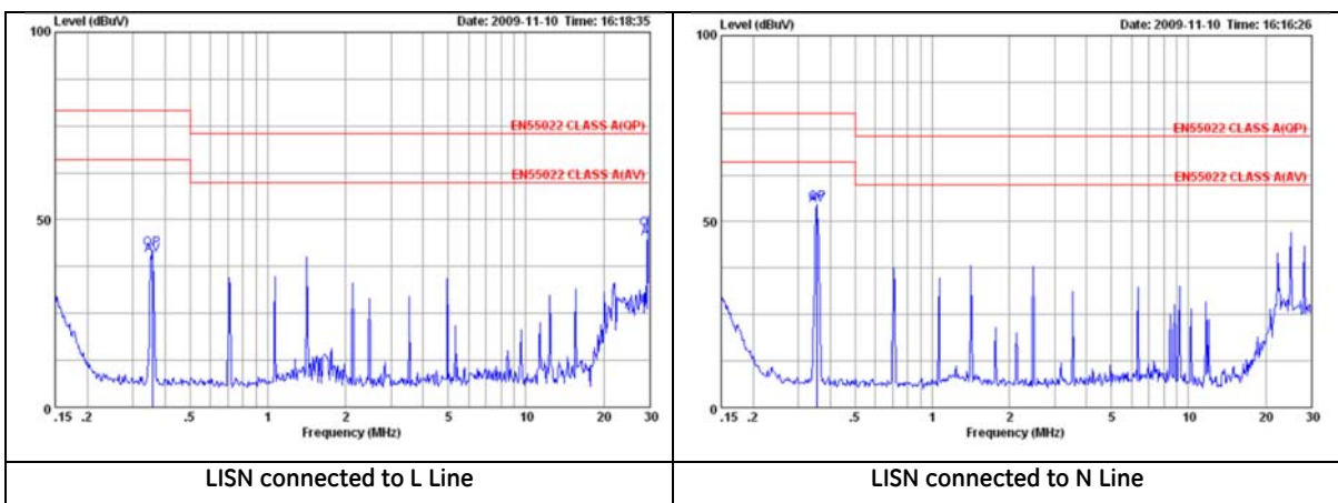
Figure 19. EMC Considerations
