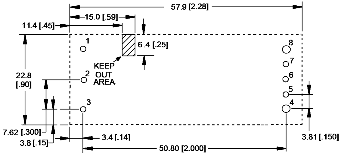
TH Recommended Pad Layout (Component Side View)
