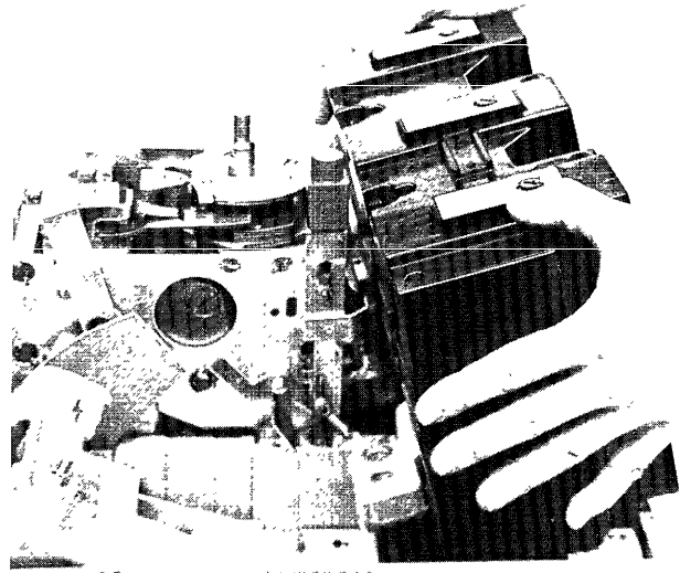
Fig. 4. Method for removal and installation of trip unit.
