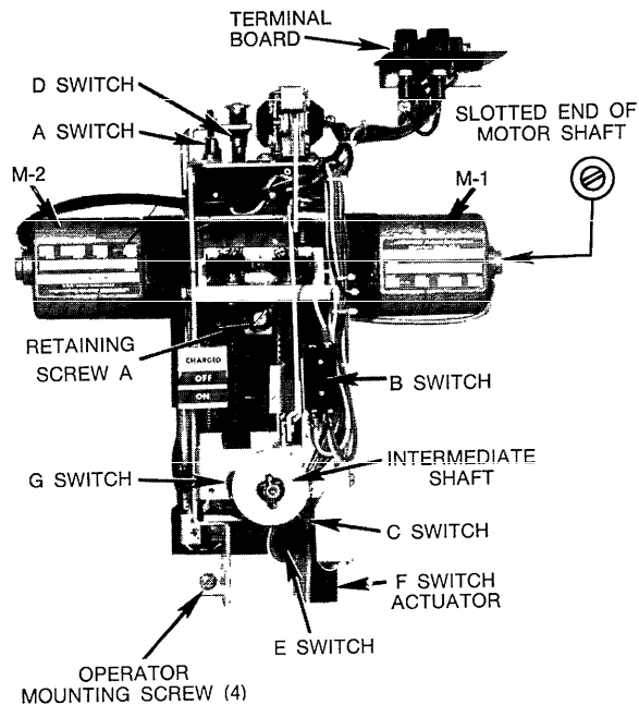
Fig. 2. Breaker with outer cover removed.
