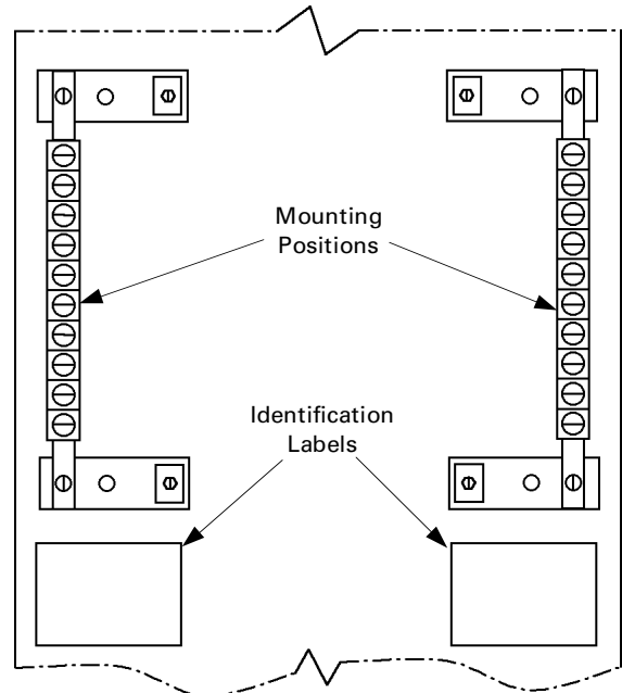
Figure 3. Equipment ground catalog number AEG21S.
