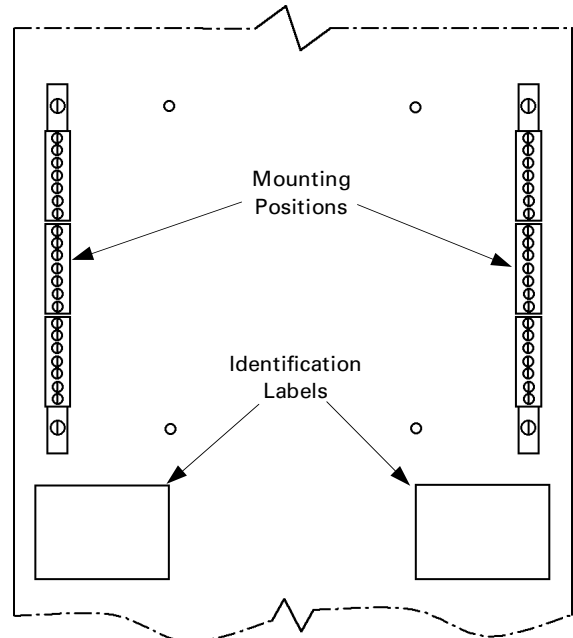
Figure 2. Equipment ground catalog number AEG21.
