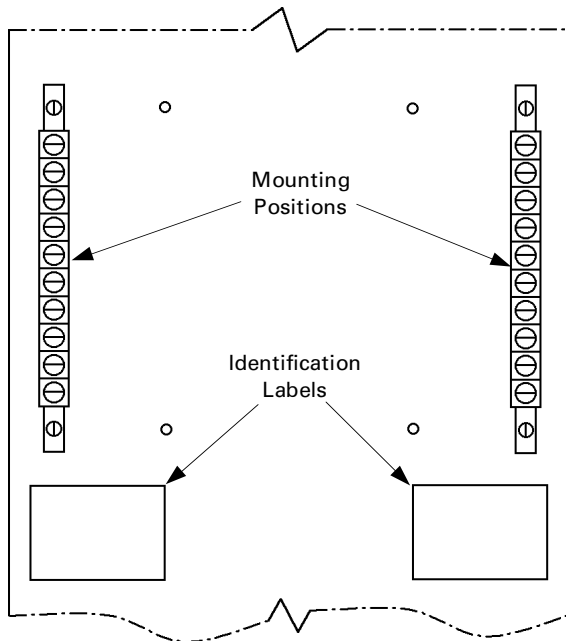
Figure 1. Equipment ground catalog number AEG10.
