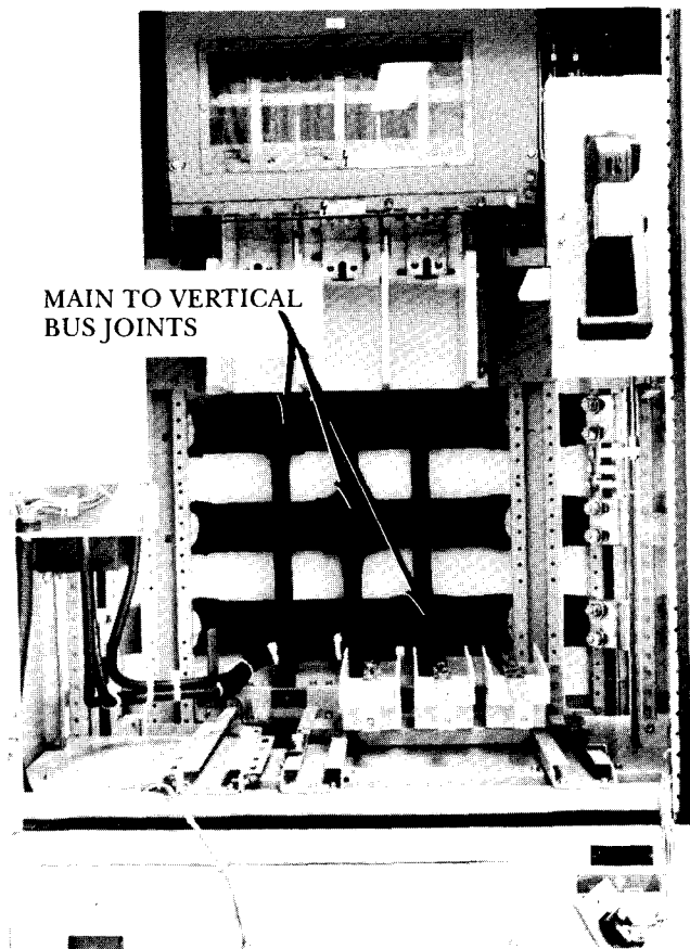
Figure 27. View of main and vertical bus area with all barriers removed (stationary contactor design)
