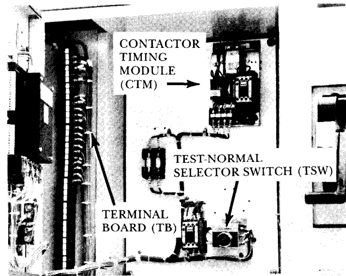
Figure 7. View of low-voltage compartment showing contactor timing module (CTM), test-normal selector switch (TSW) and terminal board (TB)
