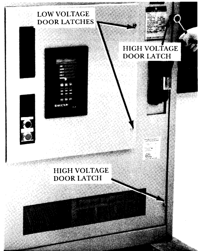
Figure 46. View showing door latch hardware
