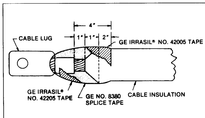
Figure 33. Termination of rubber-insulated, non-shielded, non-lead-covered, 5000-volt cable
