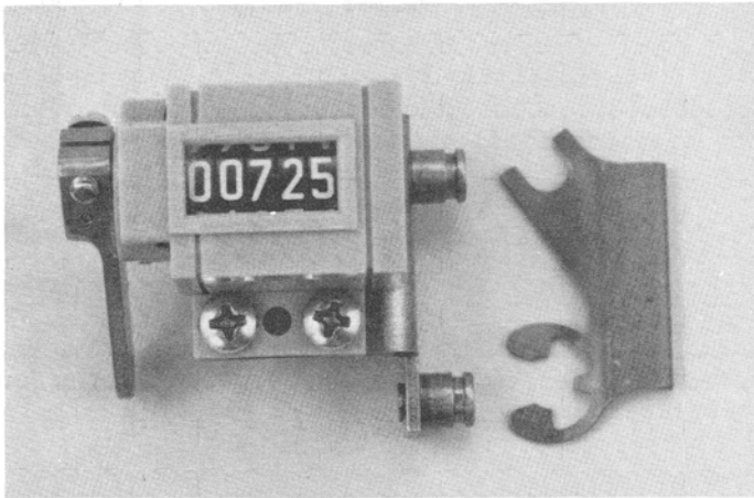
Figure 1. Mechanical Counter.
