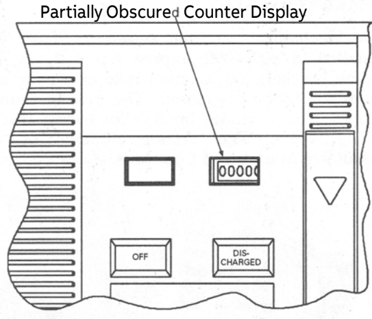
Figure 4. Counter partially obscured in top cover window.
