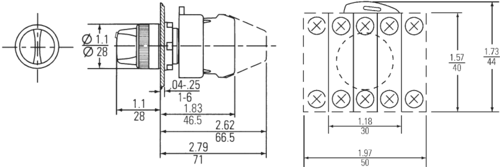
Typical Back Side View
