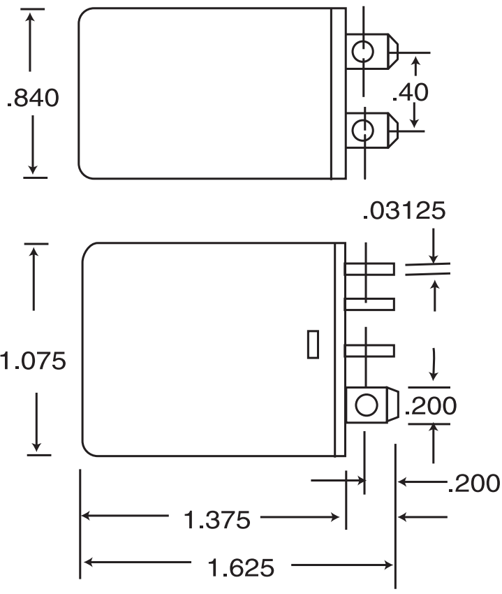
plug-in terminal
