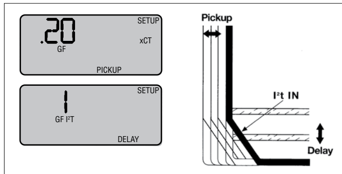
Ground fault pickup and ground fault time delay
