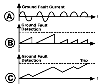
Ground fault memory circuit
