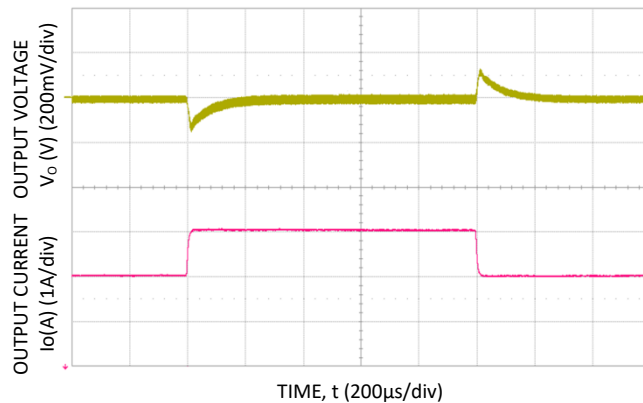
Figure 4. Transient Response to 0.1A/μs Dynamic Load Change from 50% to 75% to 50% of full load, V_{in}=24V , C_o>100μF
