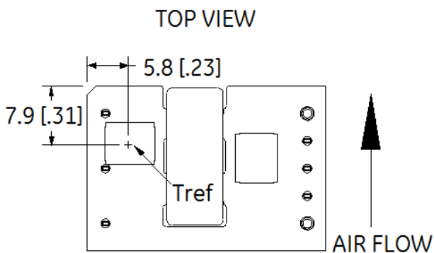
Figure 16. T_{ref} Temperature Measurement Location.
