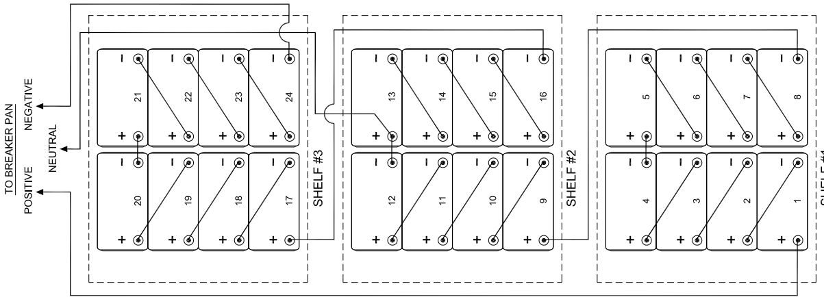
288 (+144/-144) VDC TYPICAL WIRING
