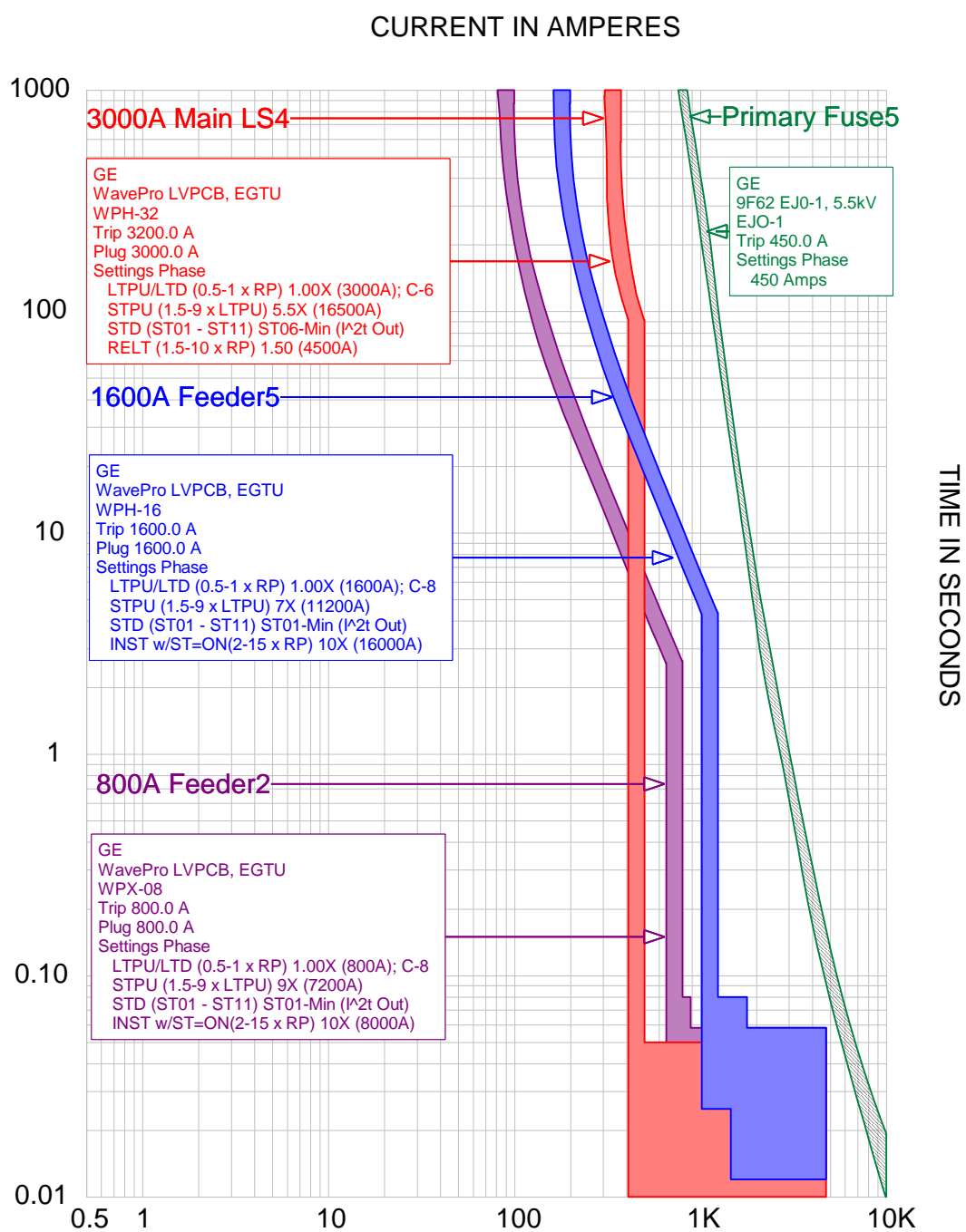
LSI-RELT (b).tcc Ref. Voltage: 480V Current in Amps x 10
