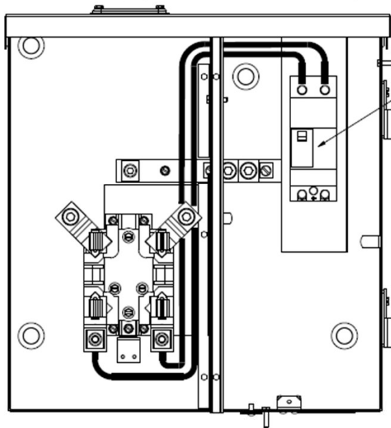
FRONT VIEW (DOORS OPEN CONDITION)
