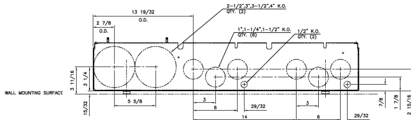
Bottom View
