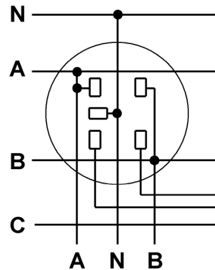
SOCKET CONNECTIONS
