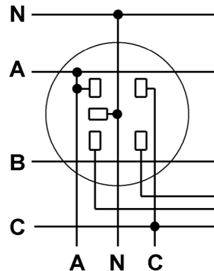
SOCKET CONNECTIONS
