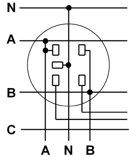
SOCKET CONNECTIONS
