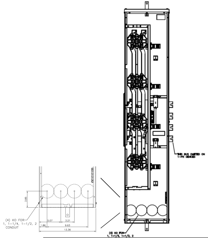
Front View
