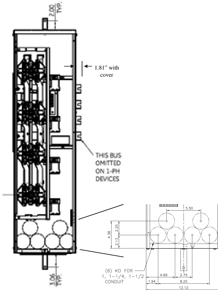
Front View
