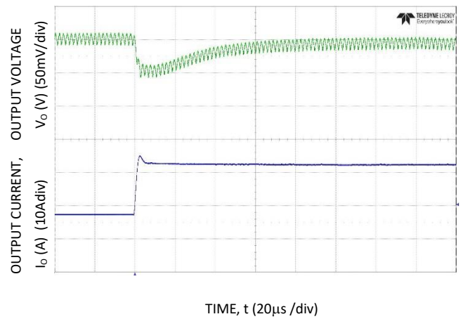
Figure 22. Transient Response to Dynamic Load Change from 50% to 100% at 12Vin, C_{out}=8x47\mu F+4x330\mu F , C_{Tune}=3300pF , R_{Tune}=221\Omega
