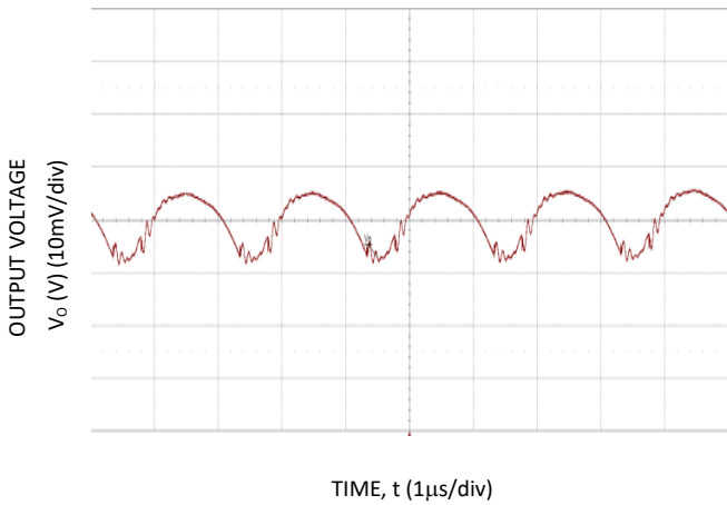
Figure 21. Typical output ripple and noise ( C_o=8x47\mu F ceramic, V_{in} = 12V , I_o = I_{o,max} ).
