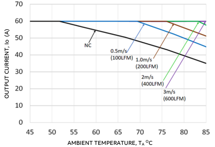
Figure 2. Derating Output Current versus Ambient Temperature and Airflow in preferred orientation.
