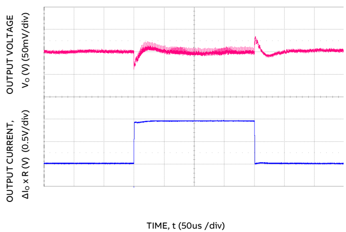
Figure 16. Transient Response to 100A/μs Dynamic Load Change from 25% to 75% at 12Vin ( C_o = 4 \times 0.1\mu F + 12 \times 47\mu F + 12 \times 1500\mu F , ASCR Gain = 256, ASCR Integrator = 128, ASCR Residual = 64). \Delta I_o = 950mV / (0.2\Omega / 7) = 33.3A
