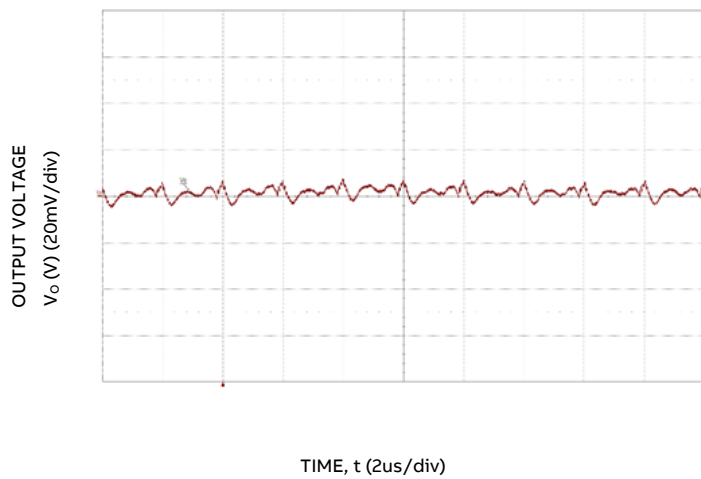
Figure 15. Typical output ripple and noise ( C_o = 4 \times 0.1\mu F + 12 \times 47\mu F + 2 \times 330\mu F polymer, V_{in} = 12V , I_o = I_{o,max} ).
