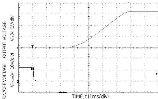
Figure 15. Typical Start-Up Using Remote On/Off with Low-ESR external capacitors ( 7 \times 150 \mu F Polymer) ( V_{in} = 12.0Vdc , V_o = 3.3Vdc , I_o = 3A , C_o = 1050 \mu F ).
