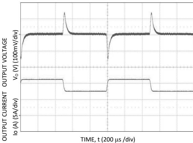
Figure 3. Transient Response to Dynamic Load Change, 1.0A/µs, from 75% to 50% to 75% of full load.
