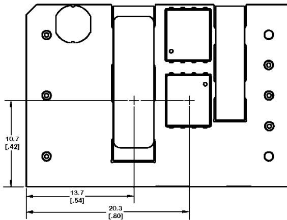
Figure 16. Pick and Place Locations.
