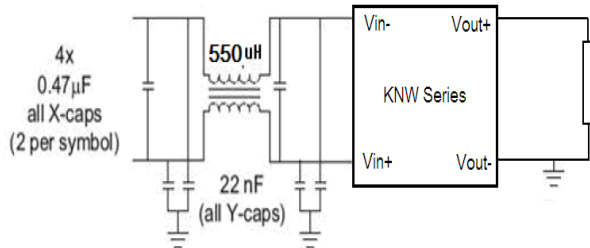
Figure 14. Single stage filter used for test results.
