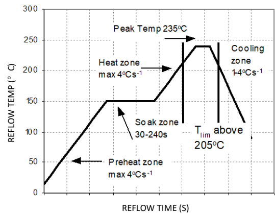
Figure 17. Reflow Profile for Tin/Lead (Sn/Pb) process
