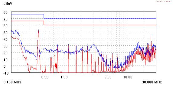
Figure 15. KNW015A0Fxx-88 Quasi Peak Conducted Emissions with EN 55022 Class A limits, Figure 14 filter ( V_{IN} = V_{IN,NOM} , I_o = 0.80 I_{o,max} ).
